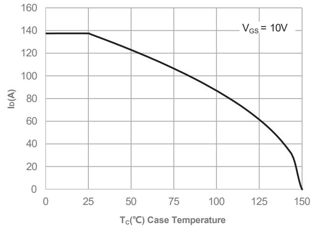
Figure 2: Current De-rating
