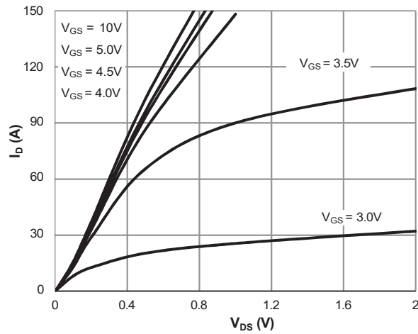
Figure 1: Saturation Characteristics
