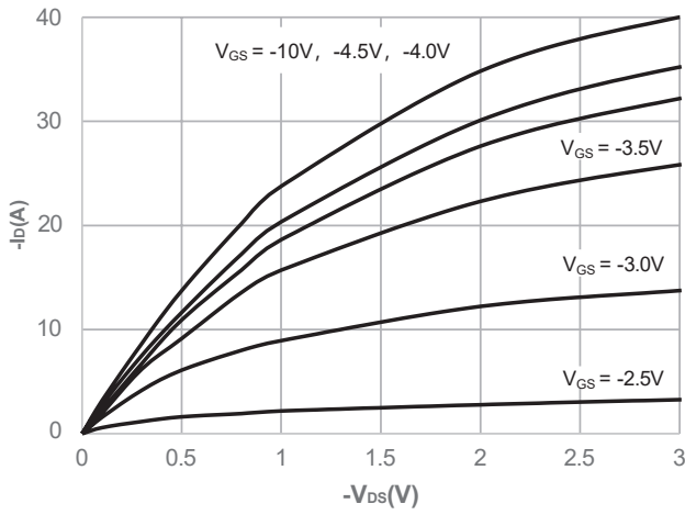
Figure 5: Output Characteristics
