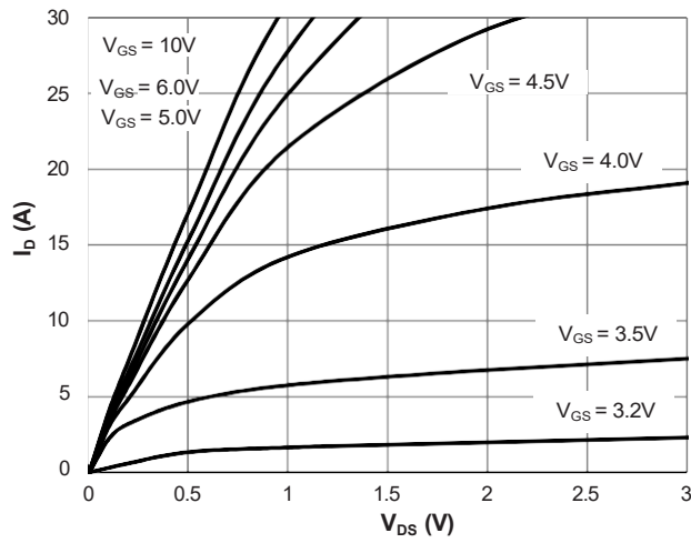
Figure 1: Saturation Characteristics
