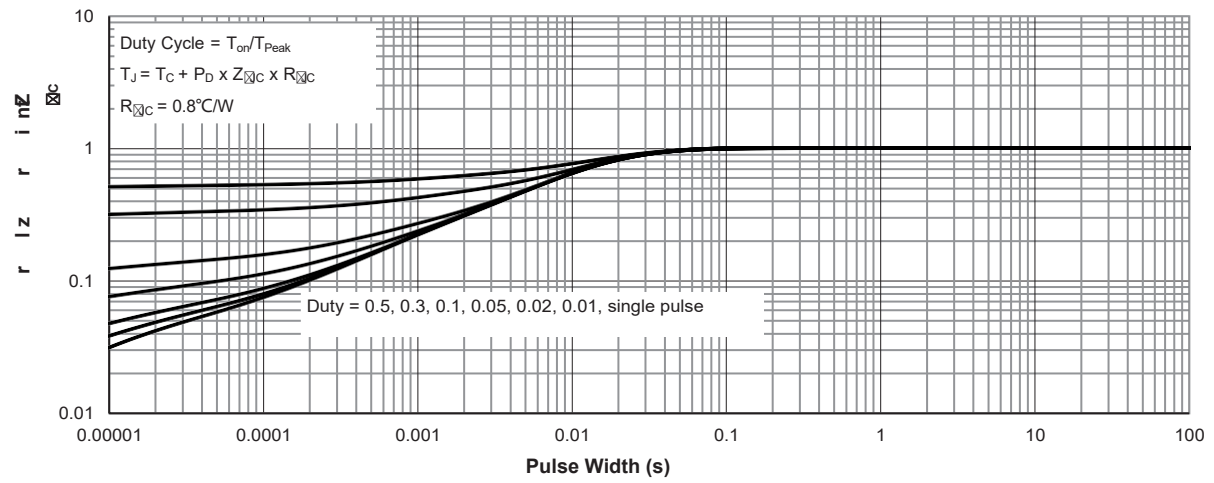
Figure 13: Normalized Transient Thermal Impedance
