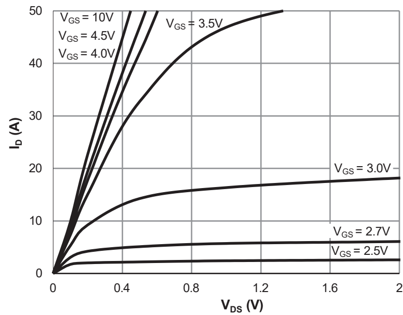
Figure 1: Saturation Characteristics
