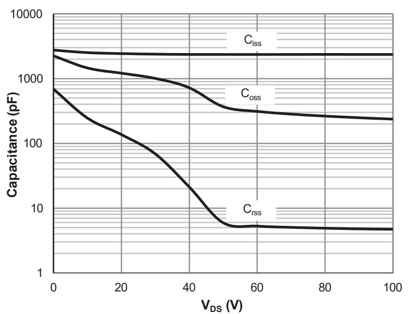
Figure 6: Capacitance Characteristics
