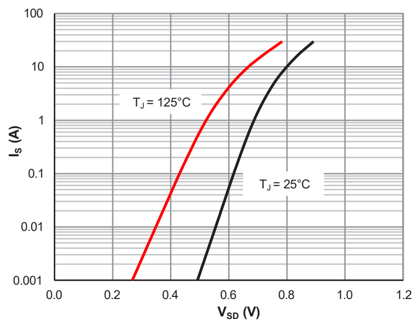
Figure 5: Body-Diode Characteristics
