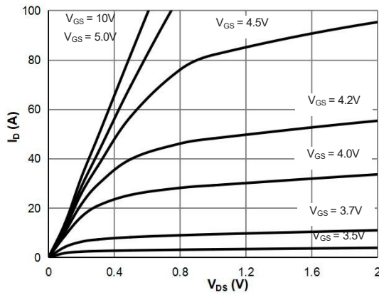
Figure 1: Saturation Characteristics
