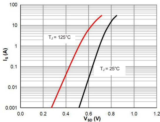
Figure 5: Body-Diode Characteristics
