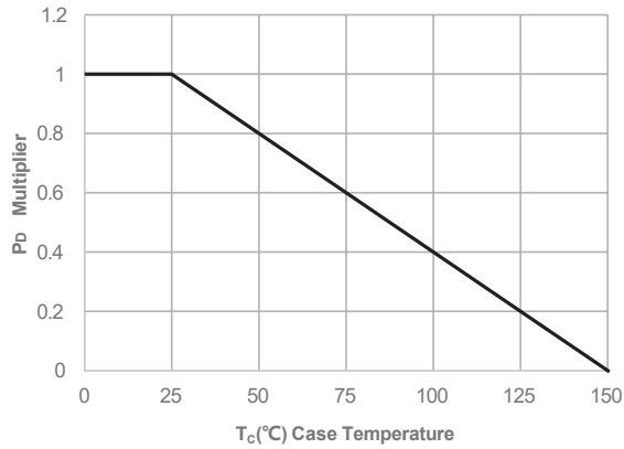
Figure 1: Power De-rating
