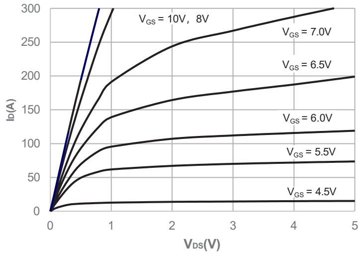
Figure 5: Output Characteristics
