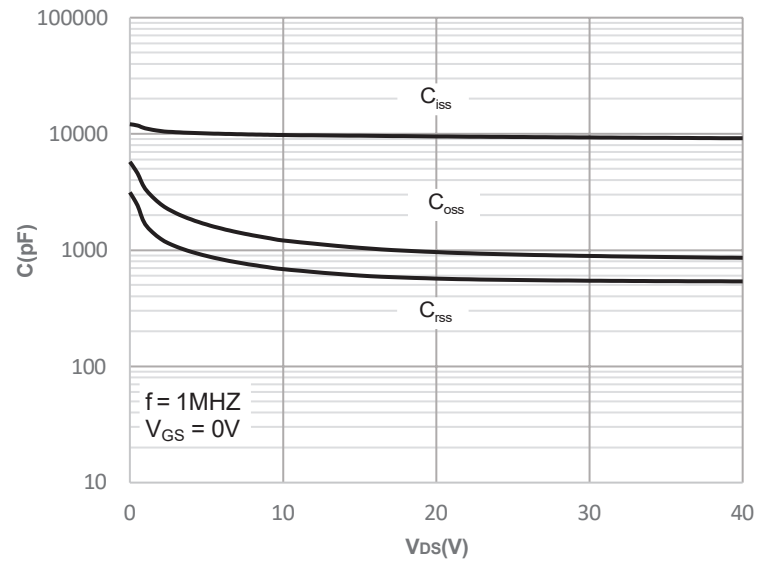
Figure 10: Capacitance Characteristics
