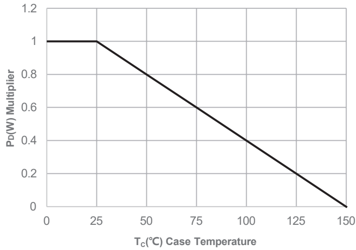
Figure 1: Power De-rating
