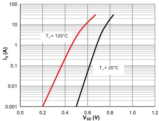
Figure 5: Body-Diode Characteristics
