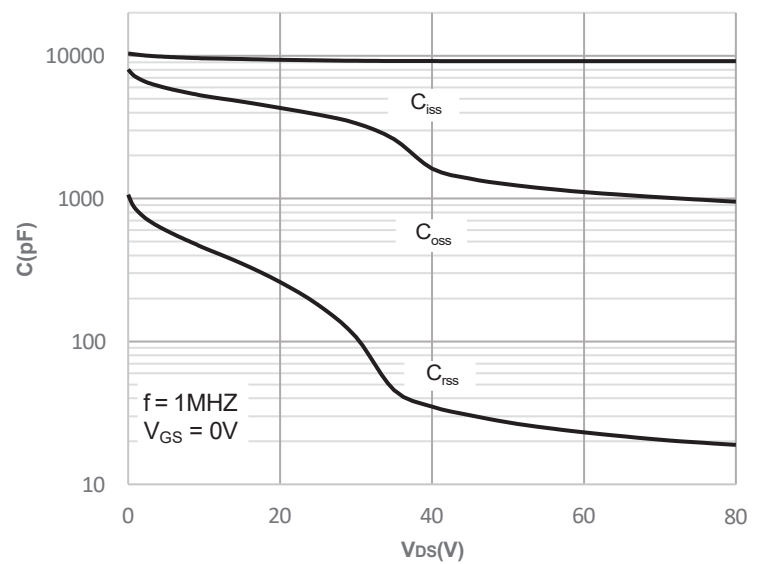
Figure 10: Capacitance Characteristics
