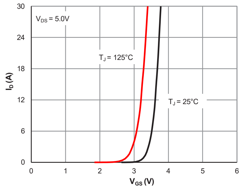
Figure 2: Transfer Characteristics
