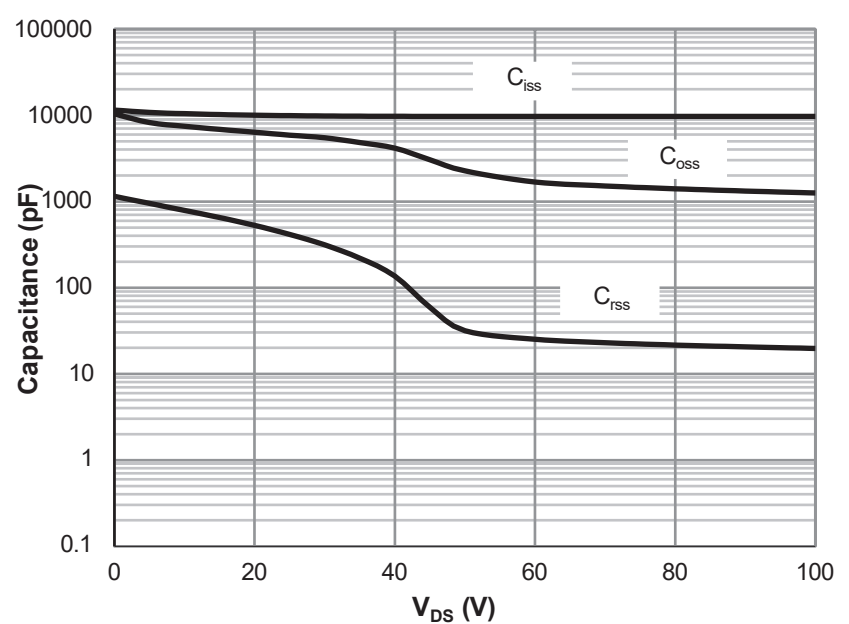
Figure 6: Capacitance Characteristics
