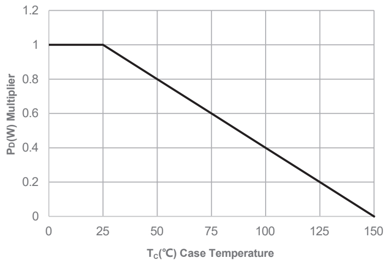
Figure 1: Power De-rating
