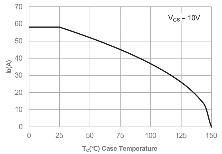
Figure 2: Current De-rating
