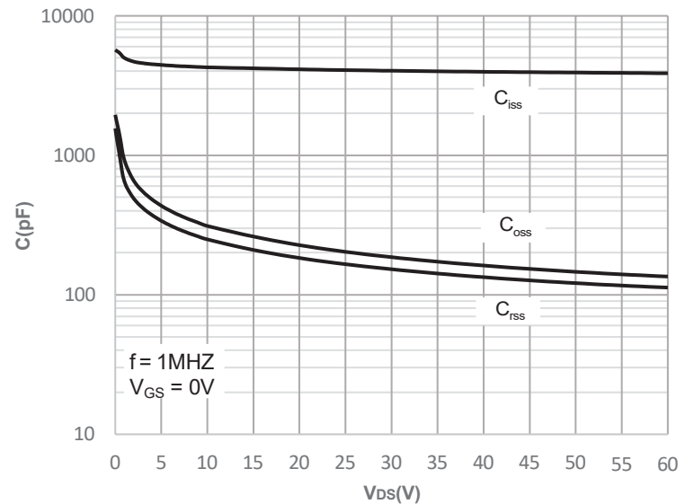
Figure 10: Capacitance Characteristics
