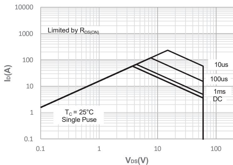
Figure 15: Maximum Safe Operating Area
