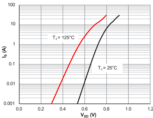
Figure 5: Body-Diode Characteristics
