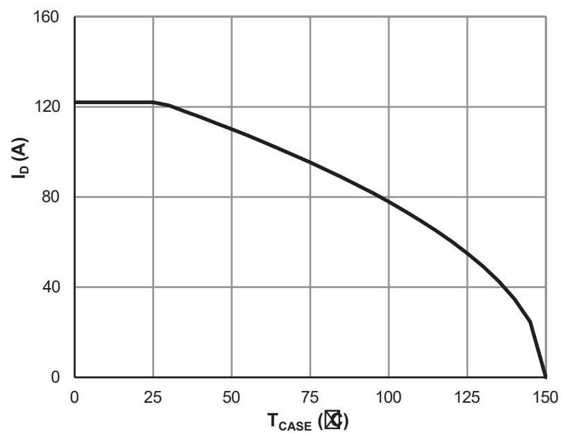
Figure 9: Current De-rating
