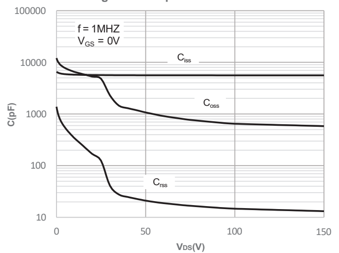
Figure 10: Capacitance Characteristics
