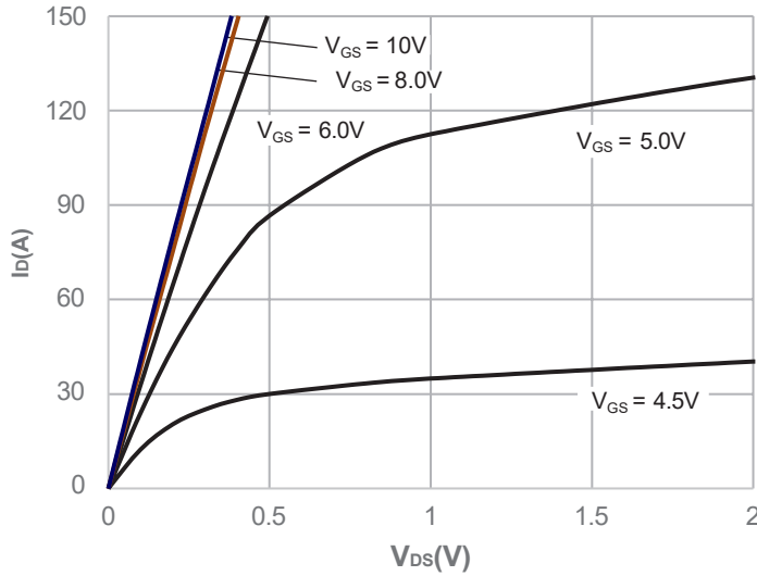
Figure 5: Output Characteristics
