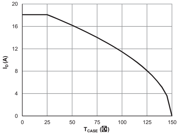
Figure 7: Current De-rating
