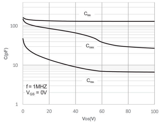
Figure 10: Capacitance Characteristics
