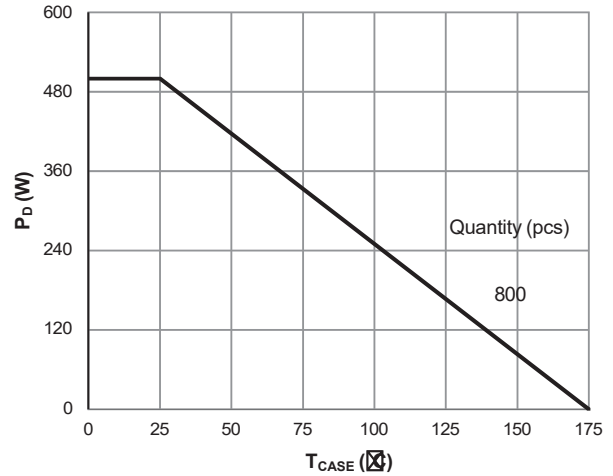
Figure 10: Power De-rating
