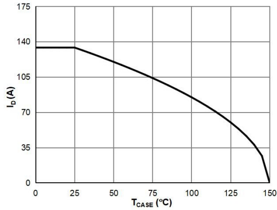
Figure 7: Current De-rating
