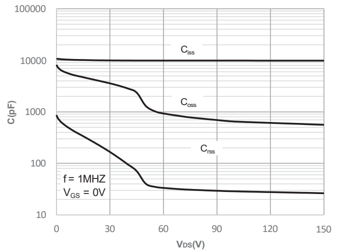
Figure 10: Capacitance Characteristics
