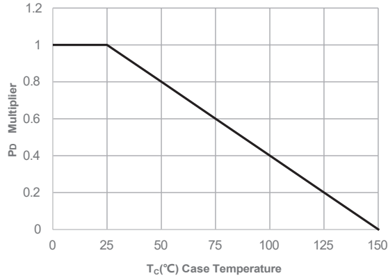
Figure 1: Power De-rating
