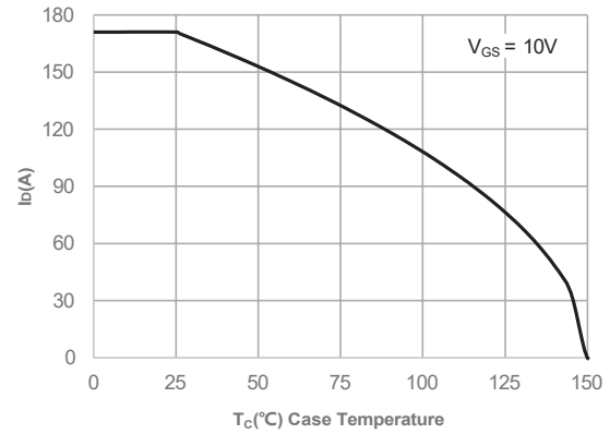
Figure 2: Current De-rating
