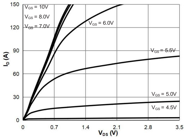
Figure 1: Saturation Characteristics
