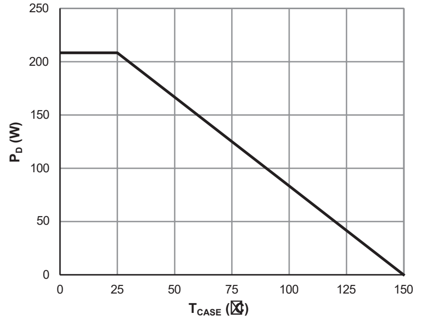
Figure 10: Power De-rating
