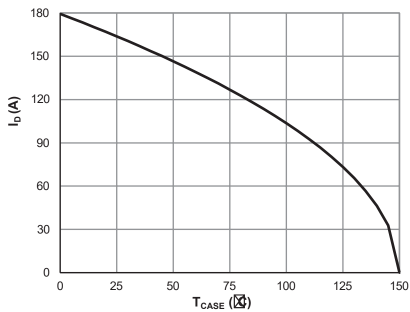
Figure 9: Current De-rating
