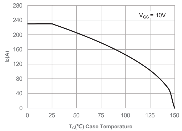
Figure 2: Current De-rating
