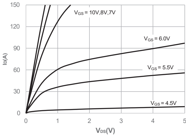
Figure 5: Output Characteristics
