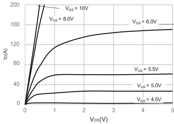
Figure 5: Output Characteristics
