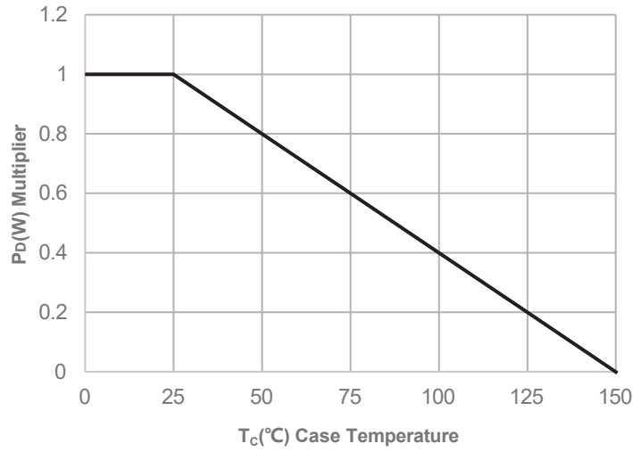
Figure 1: Power De-rating
