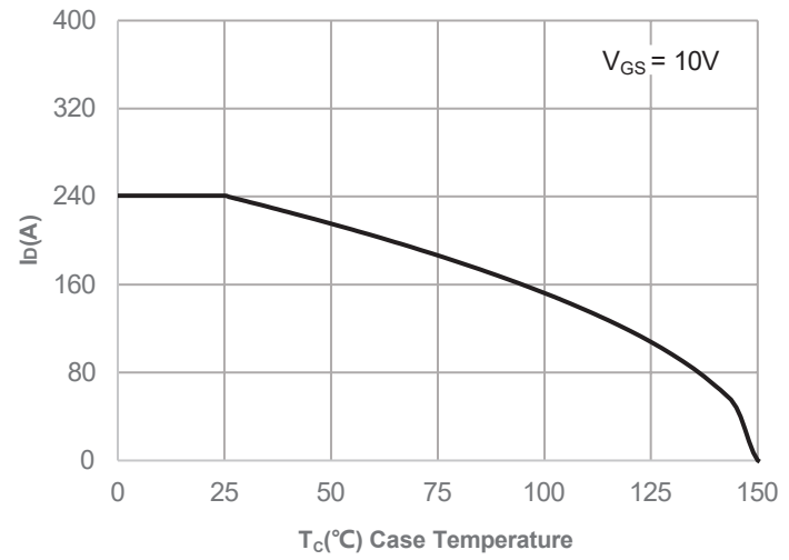
Figure 2: Current De-rating
