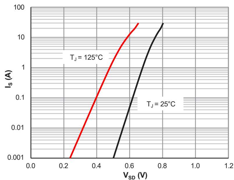
Figure 5: Body-Diode Characteristics
