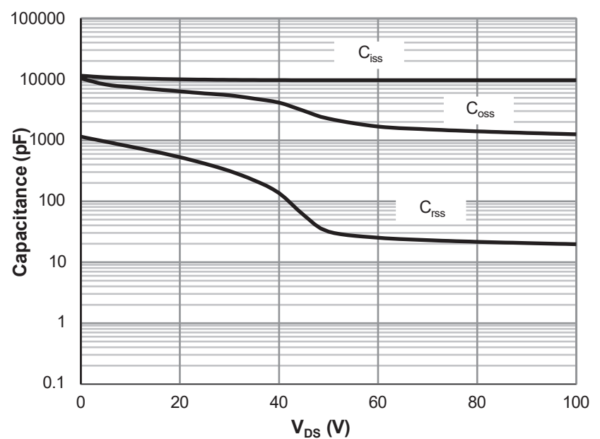
Figure 6: Capacitance Characteristics
