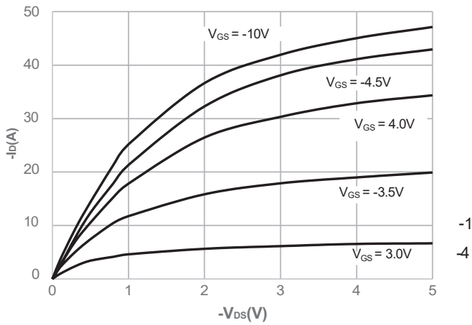
Figure 1: Output Characteristics
