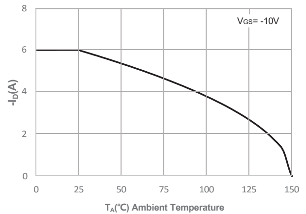
Figure 10: Maximum Continuous Driian Current vs. Ambient Temperature
