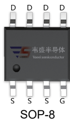
SOP-8
