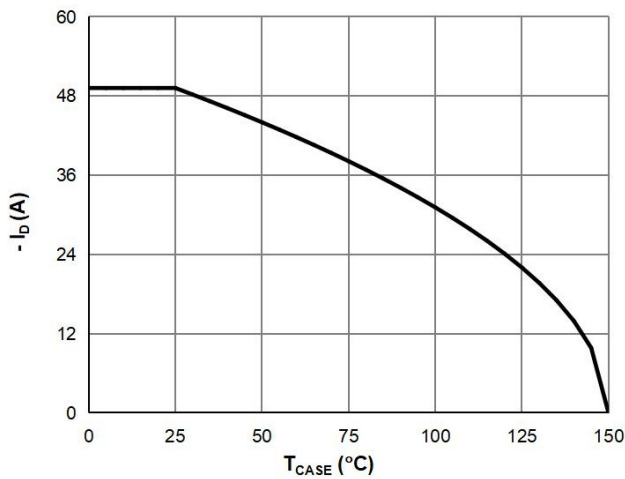
Figure 9: Current De-rating
