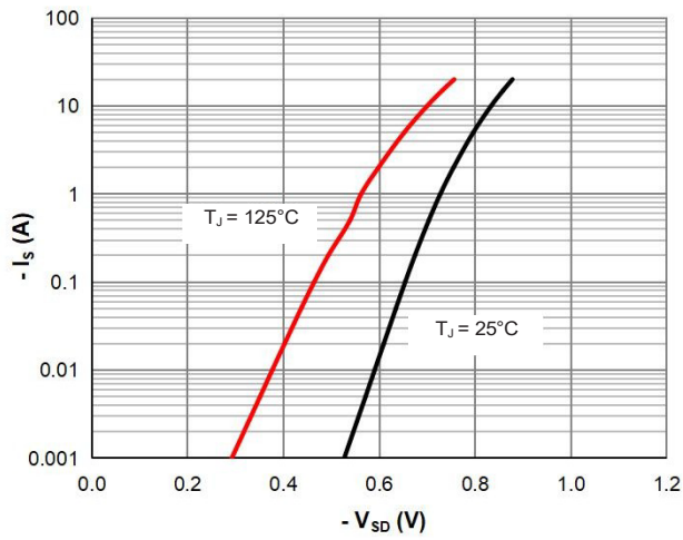
Figure 7: Body-Diode Characteristics
