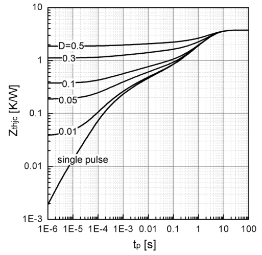
Fig 15. Transient thermal impedance, IGBT
