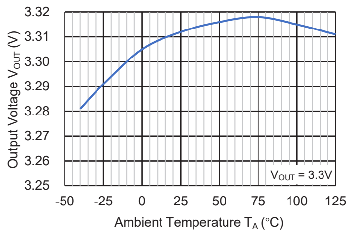
Temperature Characteristics
