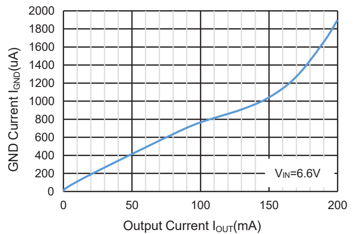
GND Current vs. Output Current
