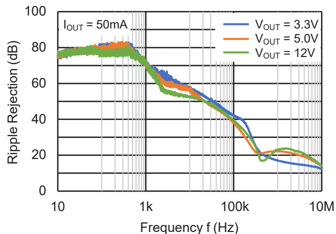
Ripple Rejection
