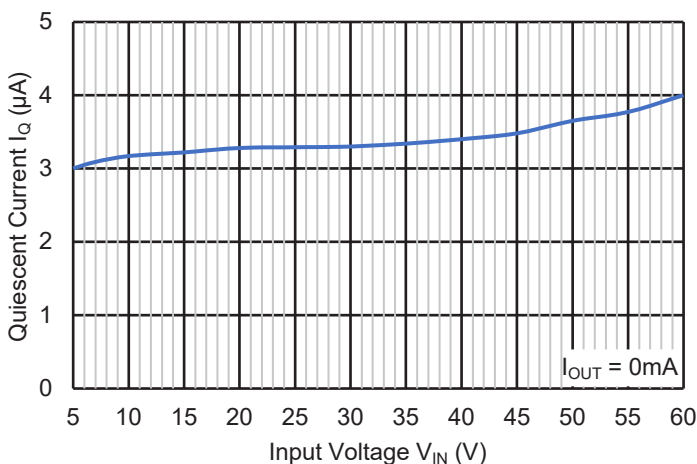
Quiescent Current
