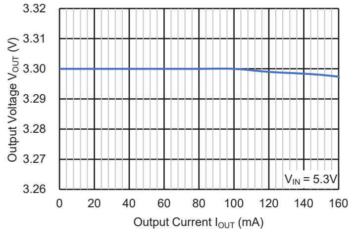
Load Regulation
