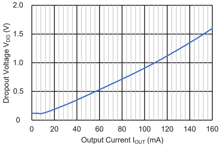
Dropout Voltage
