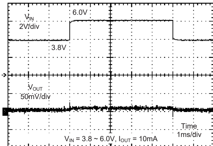
Line Transient
