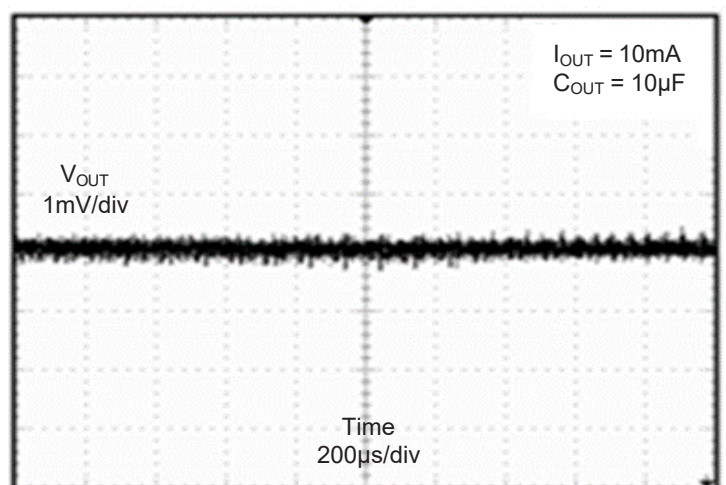
Output Noise
