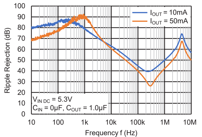
Ripple Rejection
