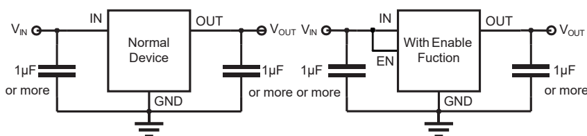
Typical Application Circuits
