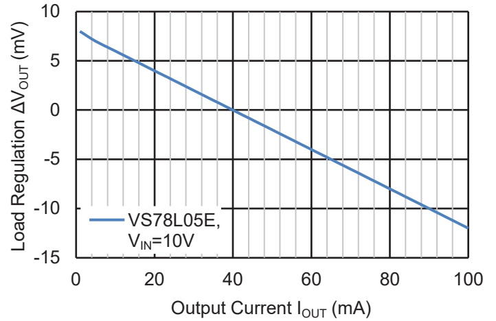
Load Regulation
