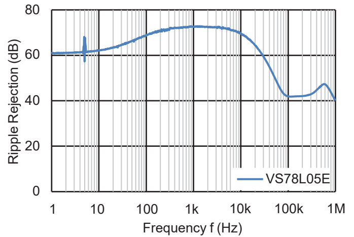
Ripple Rejection
