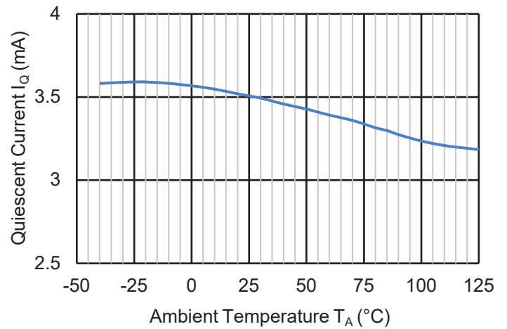
Quiescent Current
