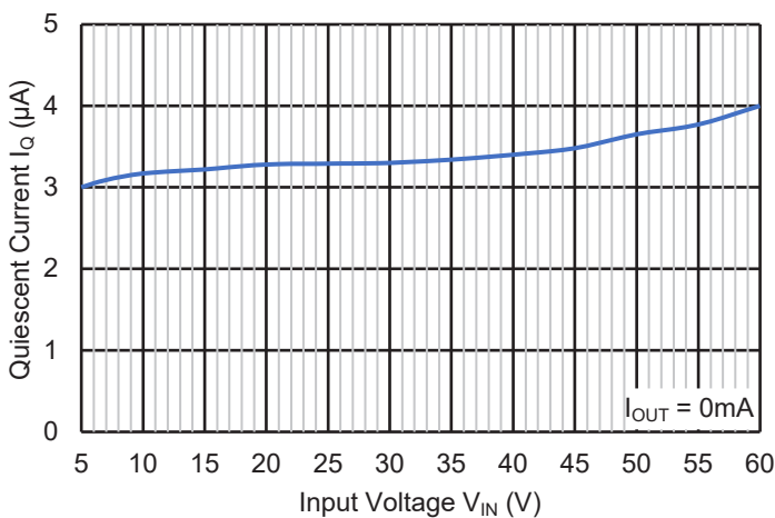
Quiescent Current
