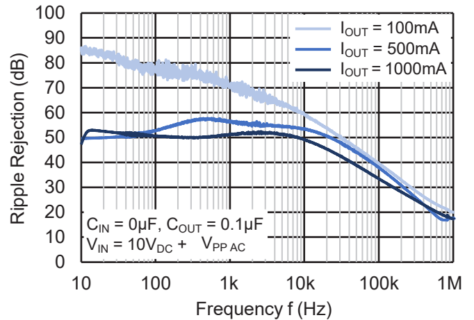
Ripple Rejection
