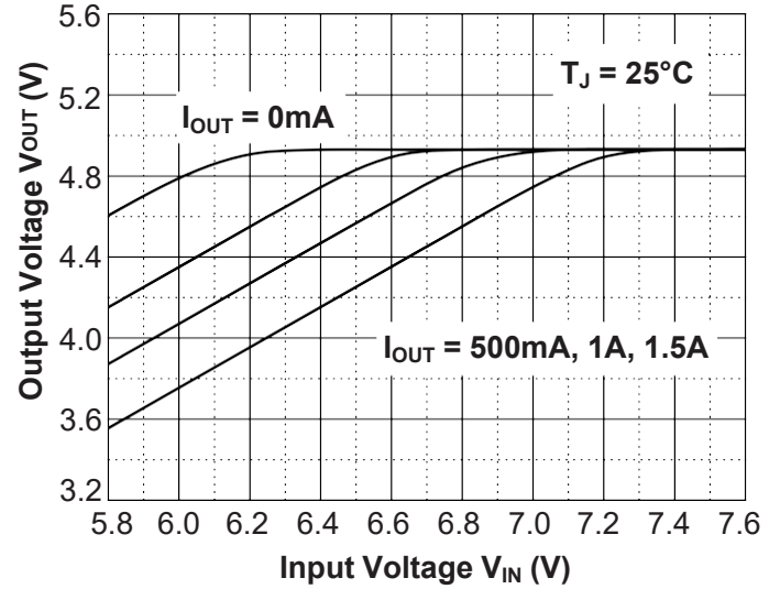
Dropout Characteristics
