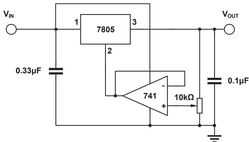
Figure 9-13. Adjustable Output
