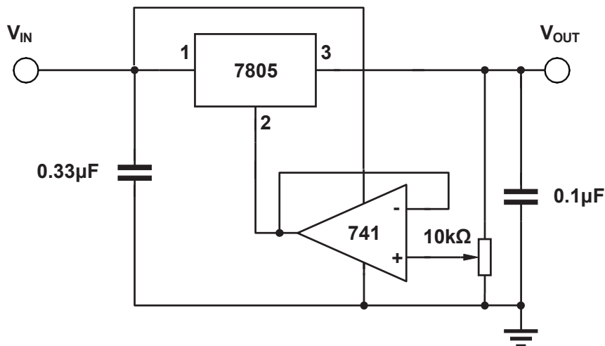
Figure 9-13. Adjustable Output
