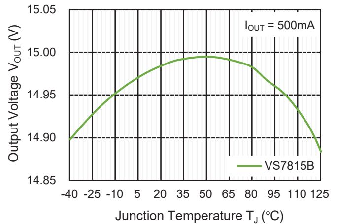
Temperature Characteristics
