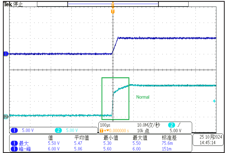
Figure 9-2. Test with the circuit that a 100μF/25V electrolytic capacitor parallel to the C_{IN} [Test Circuit is shown in Figure 9-6]
