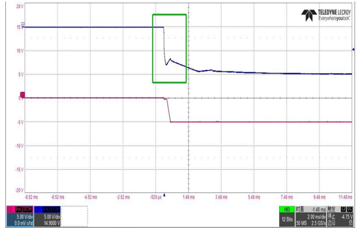
Figure 9-2. Test with the circuit that a 100\mu F/25V electrolytic capacitor parallel to the C_{IN} [Test Circuit is shown in Figure 9-6]
