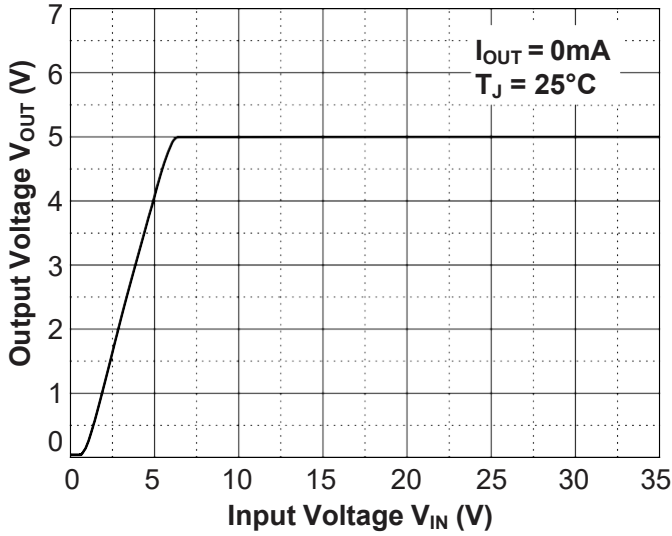
Output Characteristics
