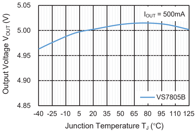
Temperature Characteristics
