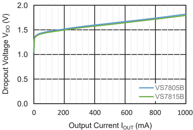
Dropout Voltage
