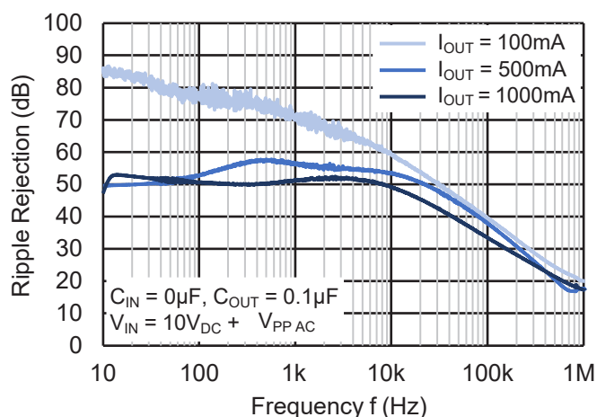
Ripple Rejection
