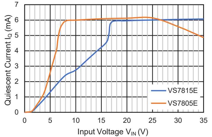
Quiescent Current
