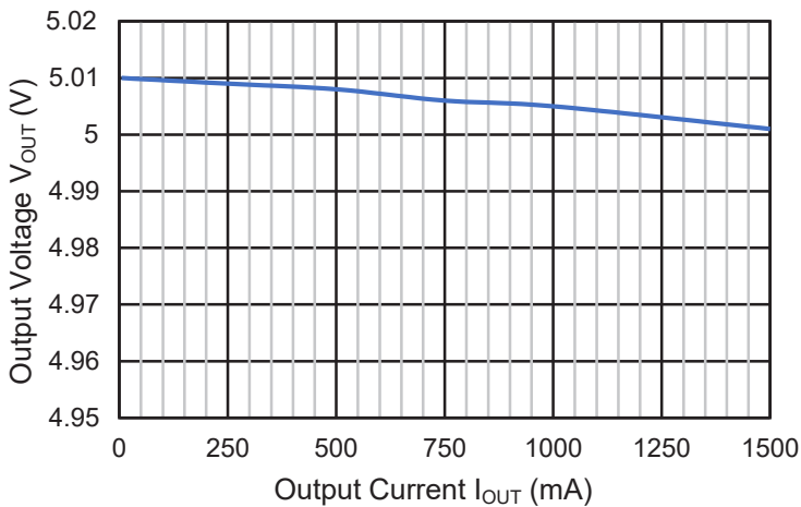
VS7805E Load Regulation
