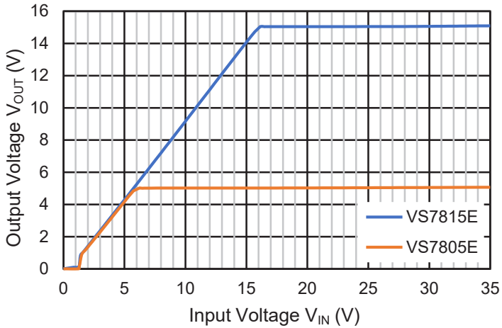
Line Regulation
