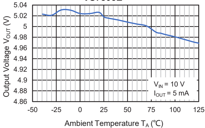
Output Voltage vs. Temperature VS7805E
