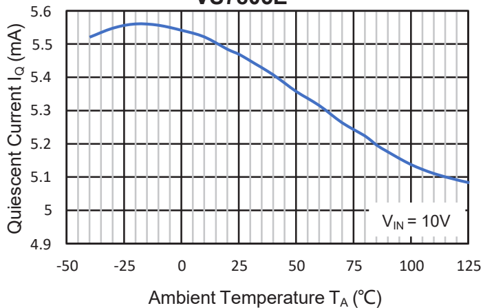
Quiescent Current vs. Temperature VS7805E
