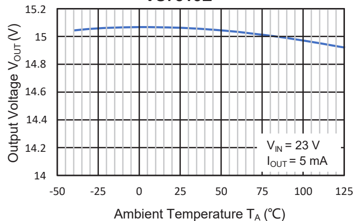
Output Voltage vs. Temperature VS7815E
