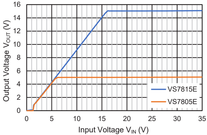
Line Regulation
