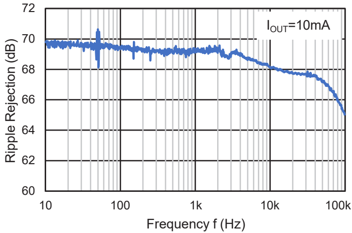
VS7805E Ripple Rejection
