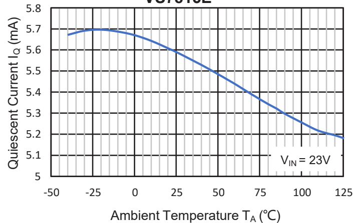
Quiescent Current vs. Temperature VS7815E
