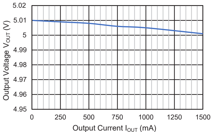
VS7805E Load Regulation
