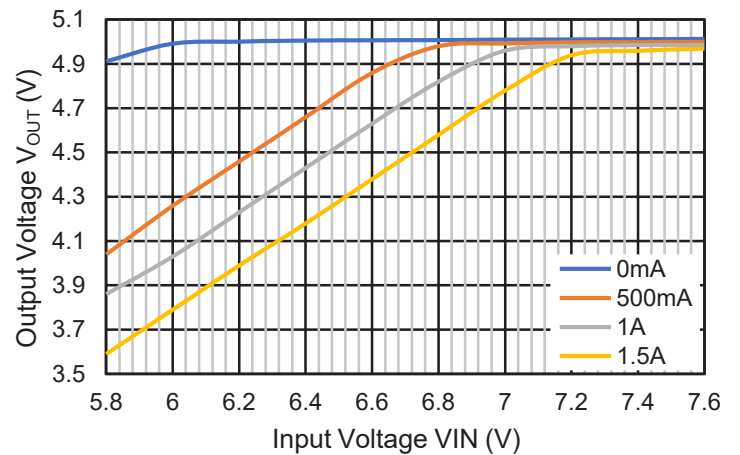
VS7805E Dropout Voltage
